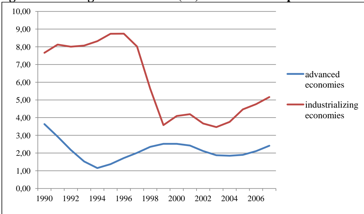
Figure 5: Average Growth rate (%) in non-ICT Capital Services
